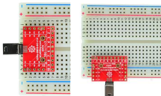
Figure 2: Example of connecting the USBm-BM10-BO-V1A on a breadboard
